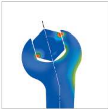
Load zones in spanners by STAHLWILLE
